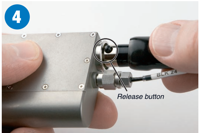
To remove the connector, pull the sleeve back to expose the black release button. Press the button to unlatch the plug.
